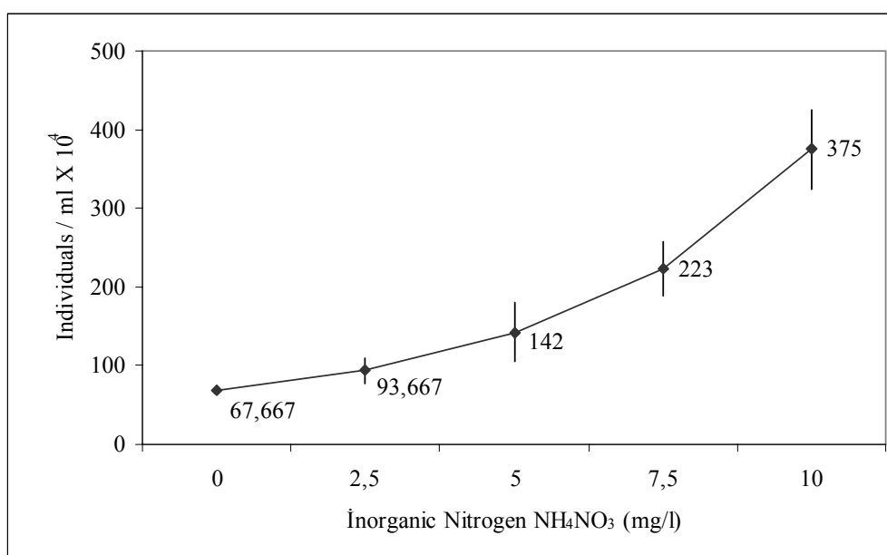
Figure 3. The growth of S. acuminatus at five different concentrations of inorganic nitrogen (NH 4 NO 3 ). Each point represents the mean ( \pm SE) individuals in three replicates of 6 day-old cultures.
