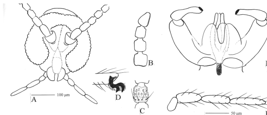
Figure 2. Lasioptera oleicola Skuhravá sp. new, male: A – head in frontal view, B – terminal part of antenna, C – fifth flagellomere, D – terminal part of the fifth tarsomere with claw and empodium, E – palpus, F - male genitalia, dorsal view. Scale below: 50 µm for B – E (Original).
