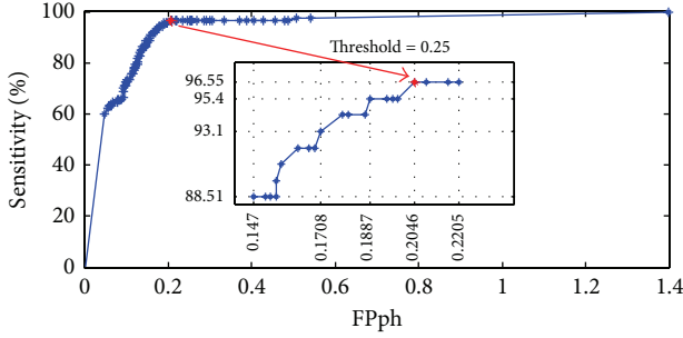
FIGURE 6: Sensitivity versus FP/h values. Best sensitivity (96.55%) for lowest FP/h (0.2046) point is marked with a red dot.
