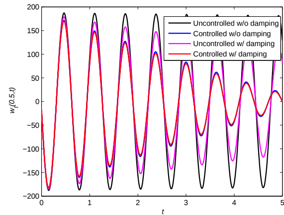
Figure 4: Controlled and uncontrolled velocities with delay at (0.5) for case a.
