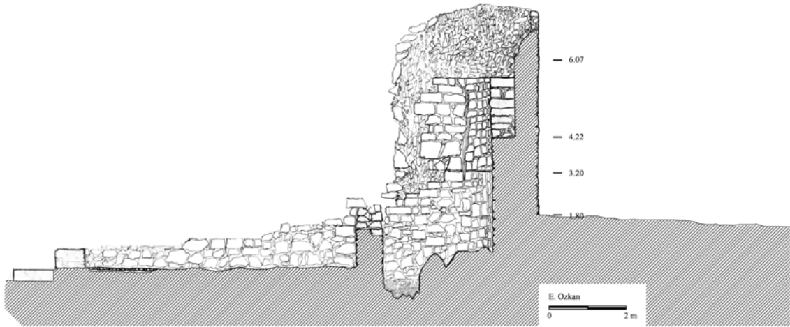
Fig. 3. Andriake Sinagog Kesiti (Çevik et al. 2010c)
