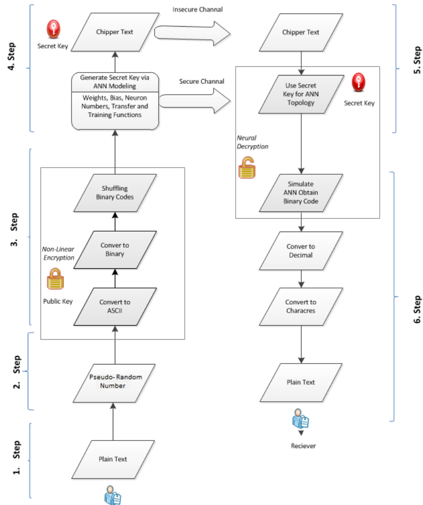
Fig. 1 Flowchart of proposed neural cryptosystem.
