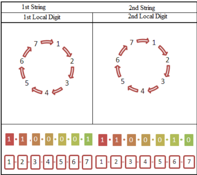
Fig. 3 Local mixing of each strings' binary codes as random times.
