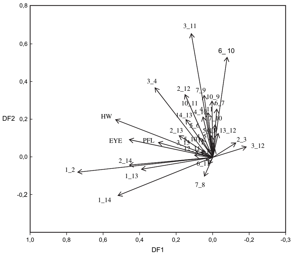
Figure 4. Contribution of morphometric variables to the canonical functions. Vectors indicate the loadings of the scores for each variable on the first two discriminant functions.
