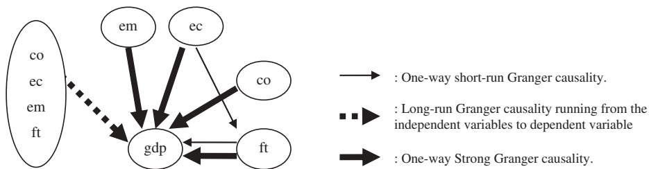
Figure 2. Granger causality relationship flows for Malta.
