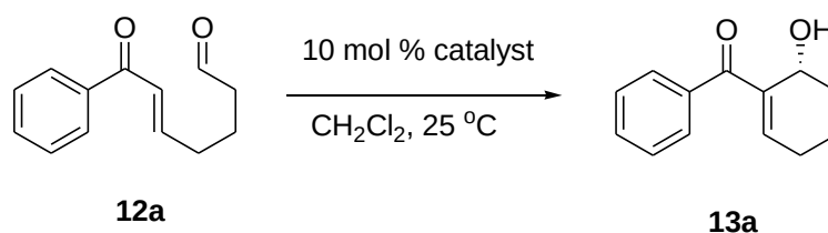
Scheme 6. Enantioselective intramolecular MBH reaction.
