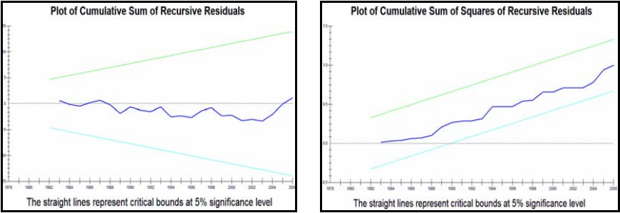
Figure 2 Plot of Cusum of Squares and Cusum test
