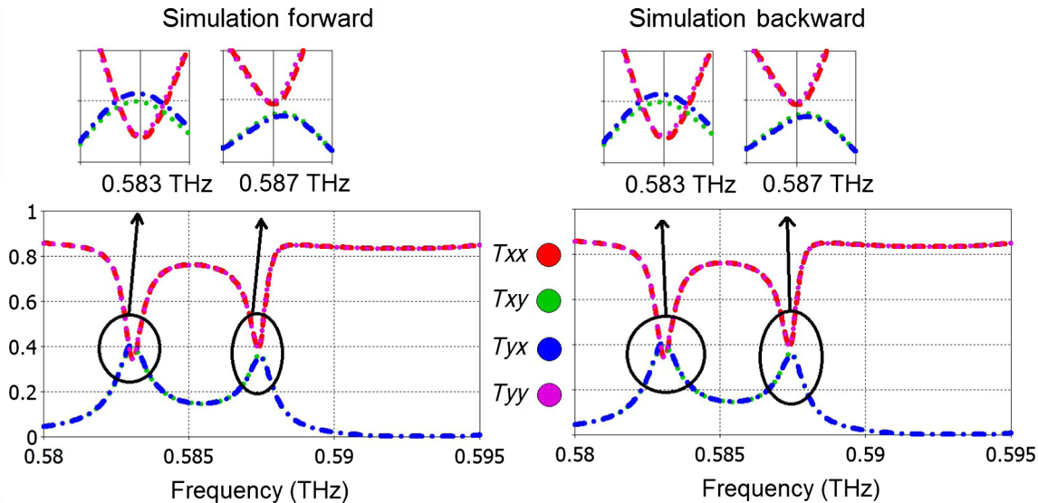
Fig. 3 Simulated transmission spectra of T -matrix elements ( T_{xx} , T_{xy} , T_{yx} and T_{yy} ) of the slab for propagations of (+z) (forward) and (−z) (backward) directions in THz.
