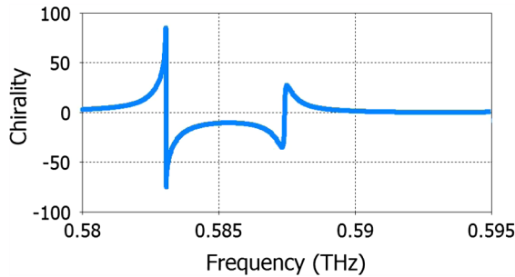
Fig. 6 Simulated chirality values of the proposed chiral MTM.
