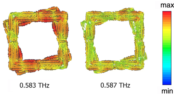
Fig. 8 Surface current distribution of the structure at the resonance frequencies.
