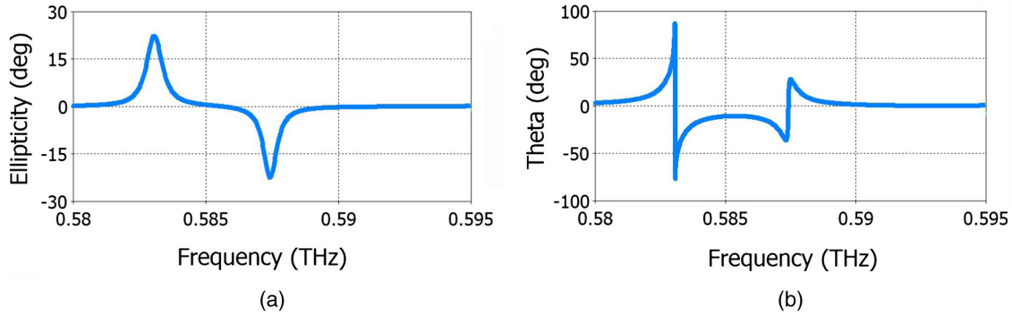
Fig. 5 Simulated circular dichroism (a) and theta degree (b) of the proposed chiral MTM.
