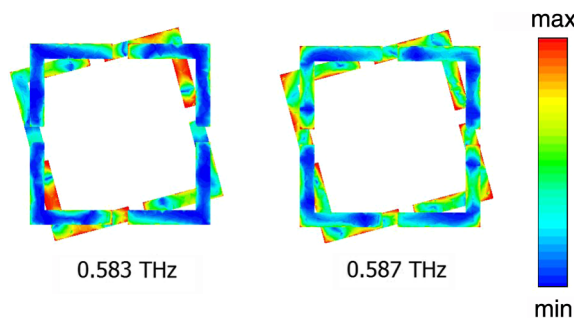
Fig. 9 Electric field distribution of the structure at the resonant frequencies.
