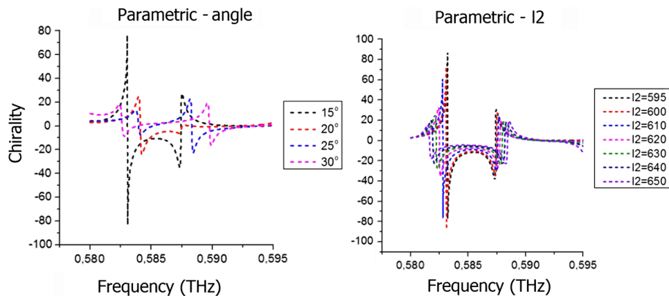
Fig. 7 Parametric numerical study results for the chirality parameter for different angles and l_2 (Fig. 1 and Table 1) wire length values.
