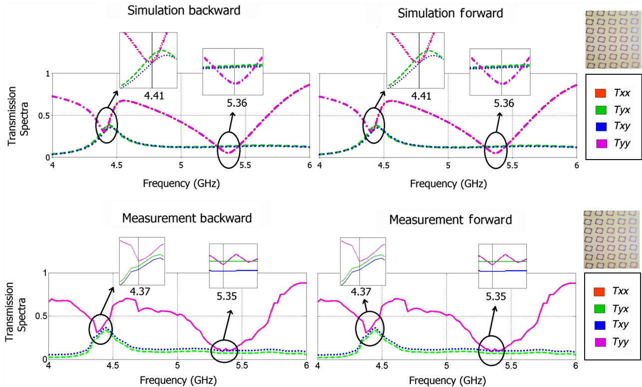
Fig. 2 Measured-simulated transmission spectra of the four matrix elements ( T_{xx} , T_{xy} , T_{yx} , T_{yy} ) of the slab for propagations in +z (f) and (b) directions in GHz. Inset: picture of the fabricated sample.
