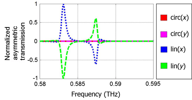
Fig. 4 Numerical results of asymmetric transmission, \Delta parameter, for linear and circular polarizations.
