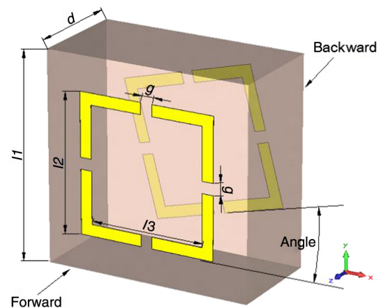
Fig. 1 The suggested chiral metamaterial (MTM) structure.
