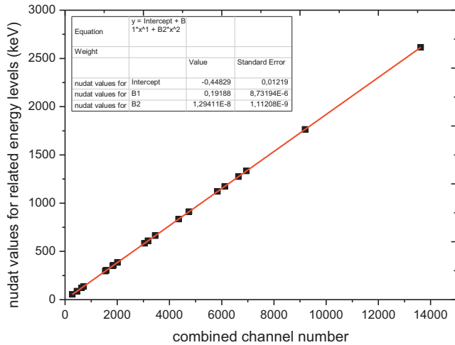
Fig. 4. Combined channel numbers for calibration point sources versus corresponding energy values taken from literature with the best values. The continuous line shows the second order polynomial fit.
