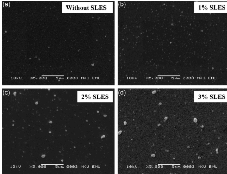
Fig. 2. Scanning electron microscopy images of the PbS films as a function of SLES concentrations in the growth solutions.
