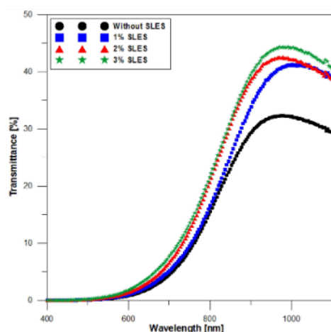
Fig. 7. UV-Vis transmittance spectra of the PbS films at different SLES concentrations.
