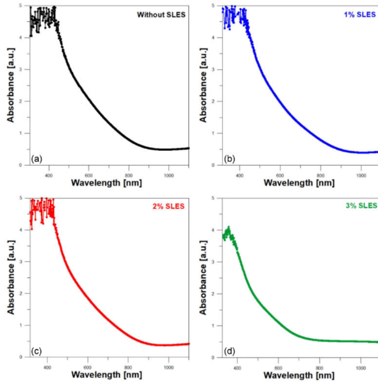
Fig. 4. UV-Vis absorbance spectra of the PbS films at different SLES concentrations (a-d).
