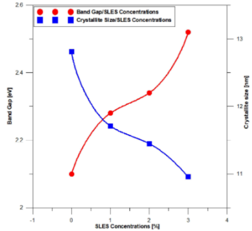
Fig. 6. Band gap and crystallite size variation as a function of SLES concentrations in the growth solutions.
