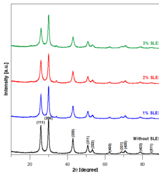
Fig. 1. X-ray diffraction patterns of the PbS films for given SLES concentrations in the growth solutions.
