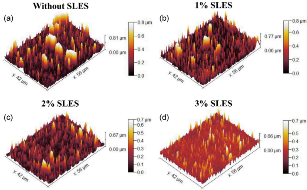
Fig. 3. SPM images of the PbS films as a function of SLES concentrations in the growth solutions (a-d).
