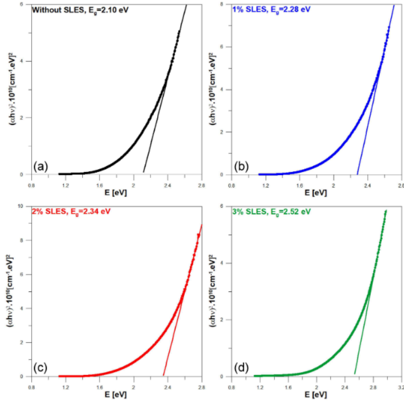
Fig. 5. Optical band gap spectra of the PbS films at different SLES concentrations (a-d).
