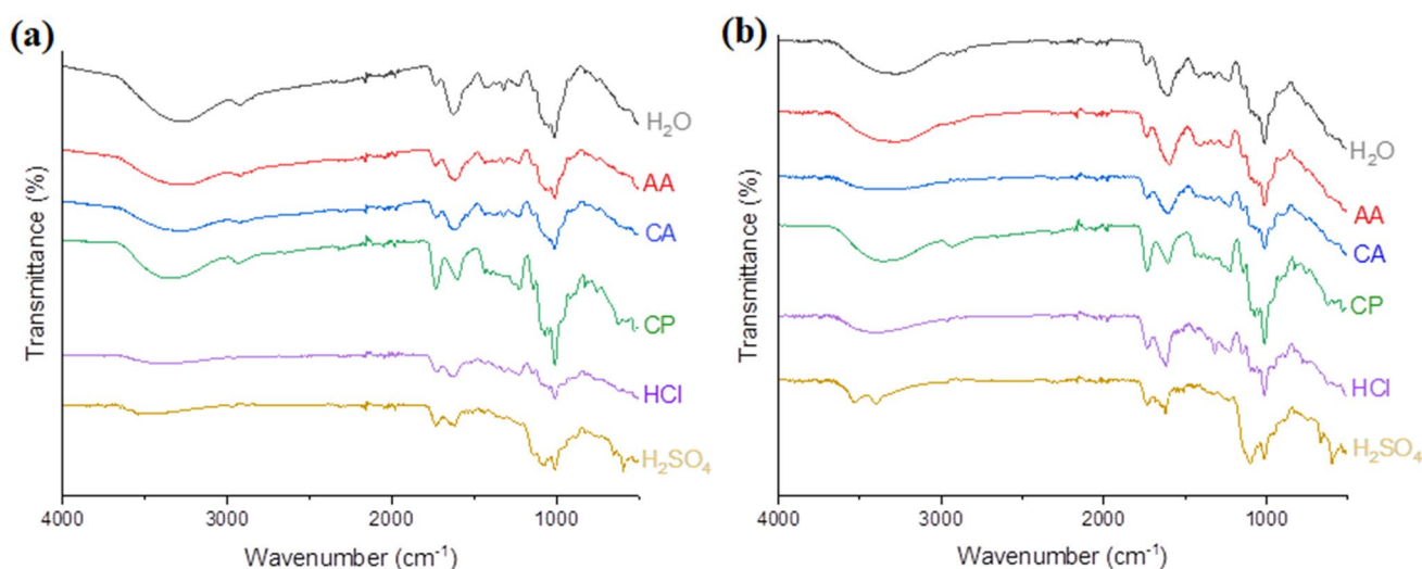
Fig. 1 FT-IR spectra results of extracted pectin from a OW, and b GW.
