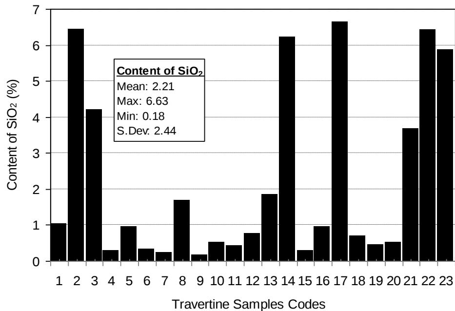
Figure 4. The histogram of SiO 2 content within travertine samples (%).
