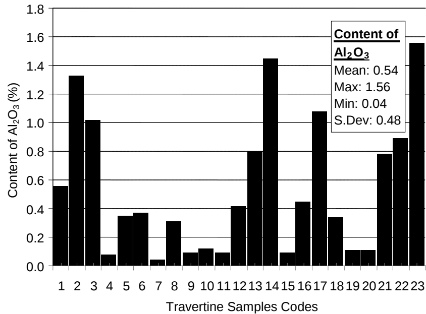
Figure 6. The histogram of \text{Al}_2\text{O}_3 content within travertine samples (%).
