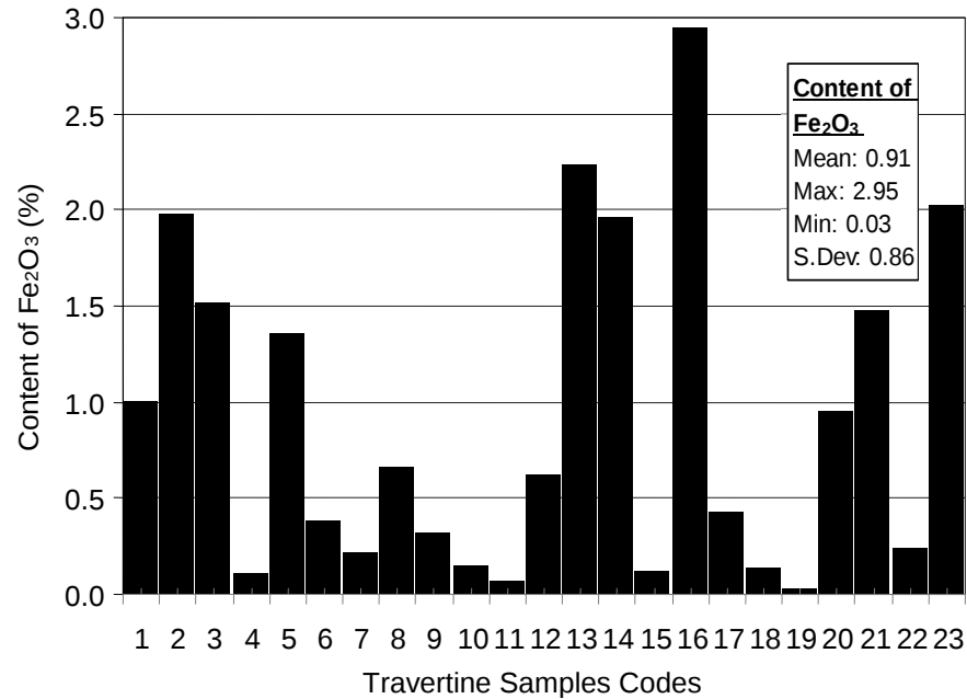
Figure 5. The histogram of \text{Fe}_2\text{O}_3 content within travertine samples (%).
