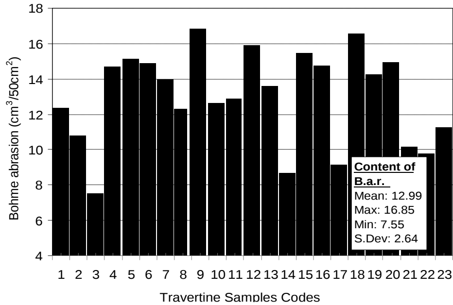
Figure 16. The histogram of Bohme abrasion within travertine samples ( \text{cm}^3/50\text{cm}^2 ).
