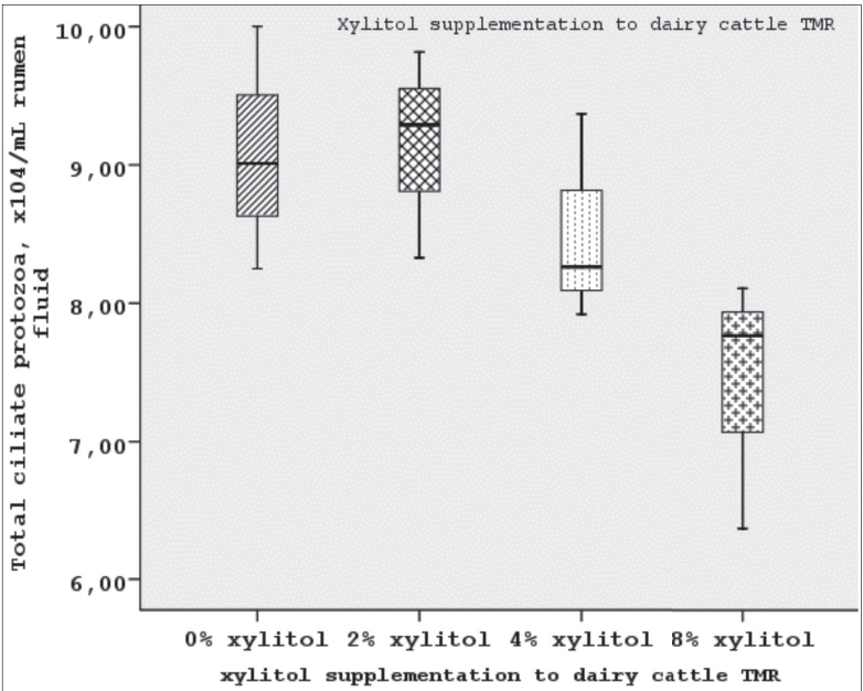
Fig 2. Total ciliate protozoa number of ruminal fluid the in vitro fermentation for dairy cattle TMR with xylitol supplementation (P values; Linear: 0.815 and Quadratic: 0.188)
